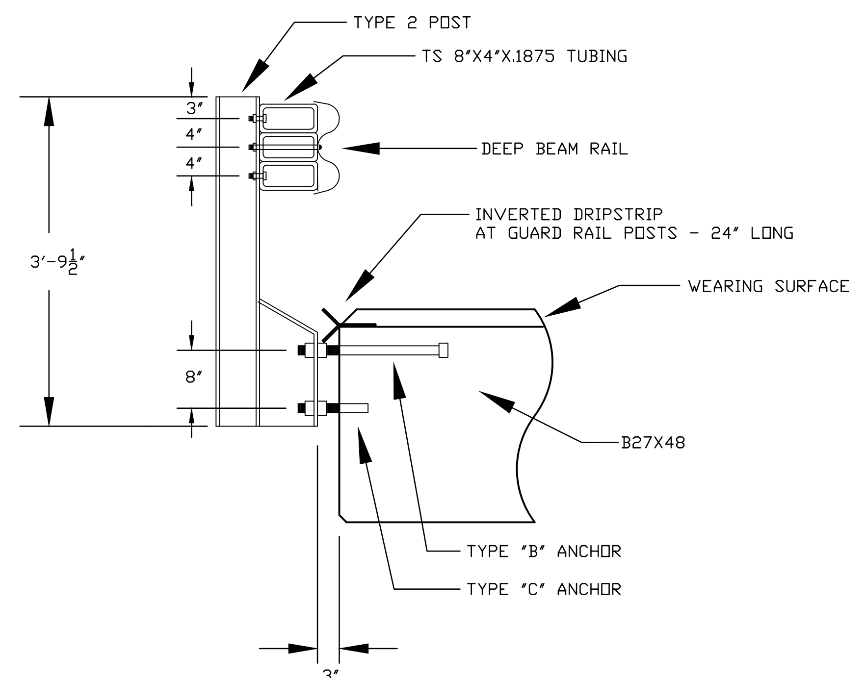
GUARDRAIL DETAIL
