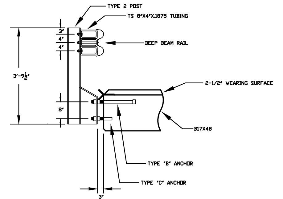
GUARDRAIL DETAIL
